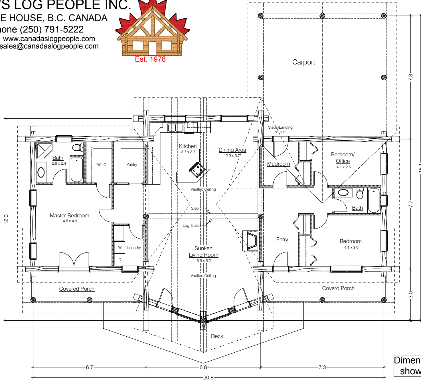
Main Floor Plan 192.3 Sq. M.
